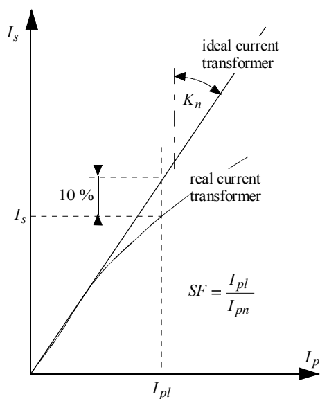
Figure 6-11: safety factor ( SF ) of measuring CTs
