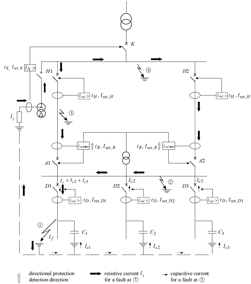
Figure 10-14: neutral earthing via resistance on the busbar
