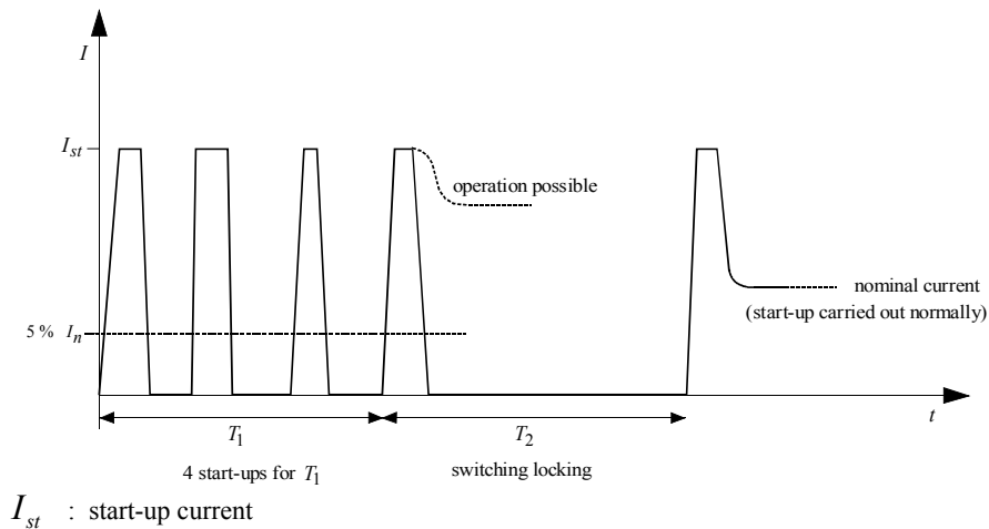
Figure 7-57: a successive number of start-ups above the limiting value
