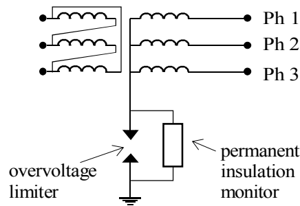
Figure 2-11: installation of an overvoltage limiter and a permanent insulation monitor in an IT system
