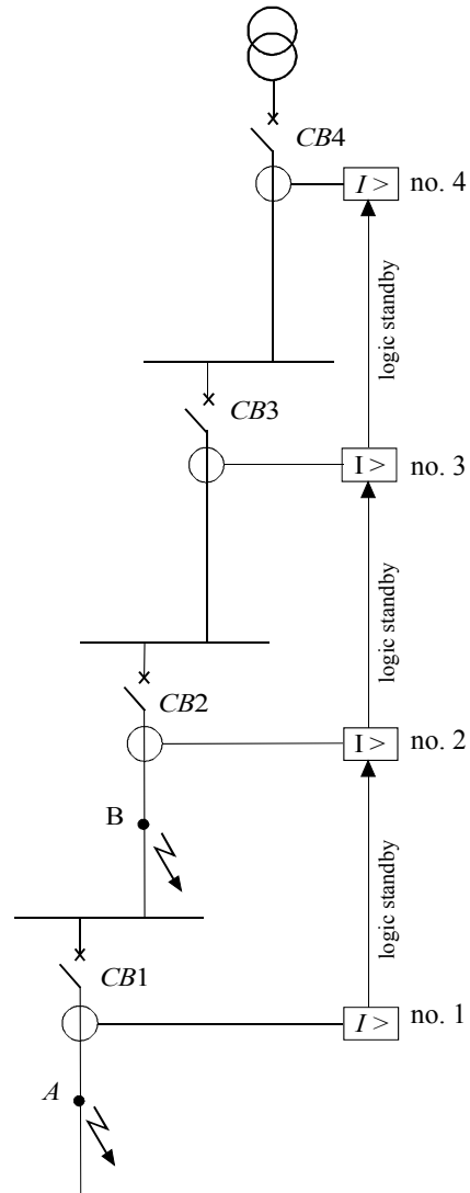
Figure 9-6: logic selectivity
