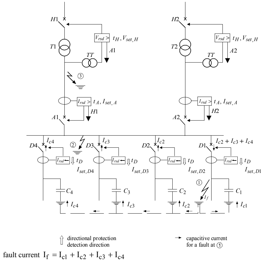
Figure 10-11: unearthed neutral
