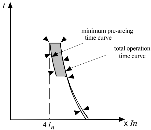
Figure 8-11: standardized fusing zones for a gM fuse
