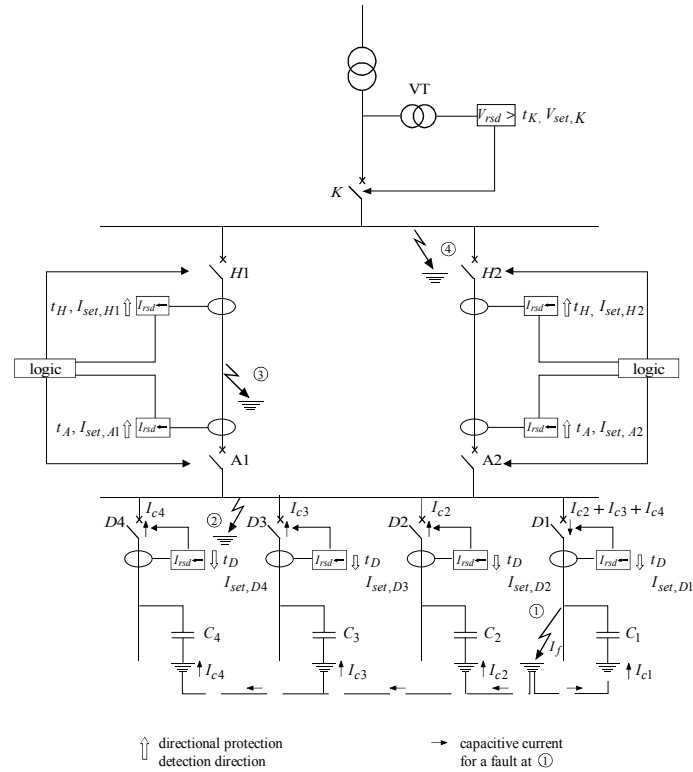
Figure 10-15: unearthed neutral
