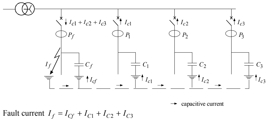
Figure 7-22: distinguishing between a fault current and a capacitive current in an ungrounded neutral system
