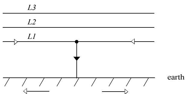
Figure 3-1: phase-to-earth short-circuit
