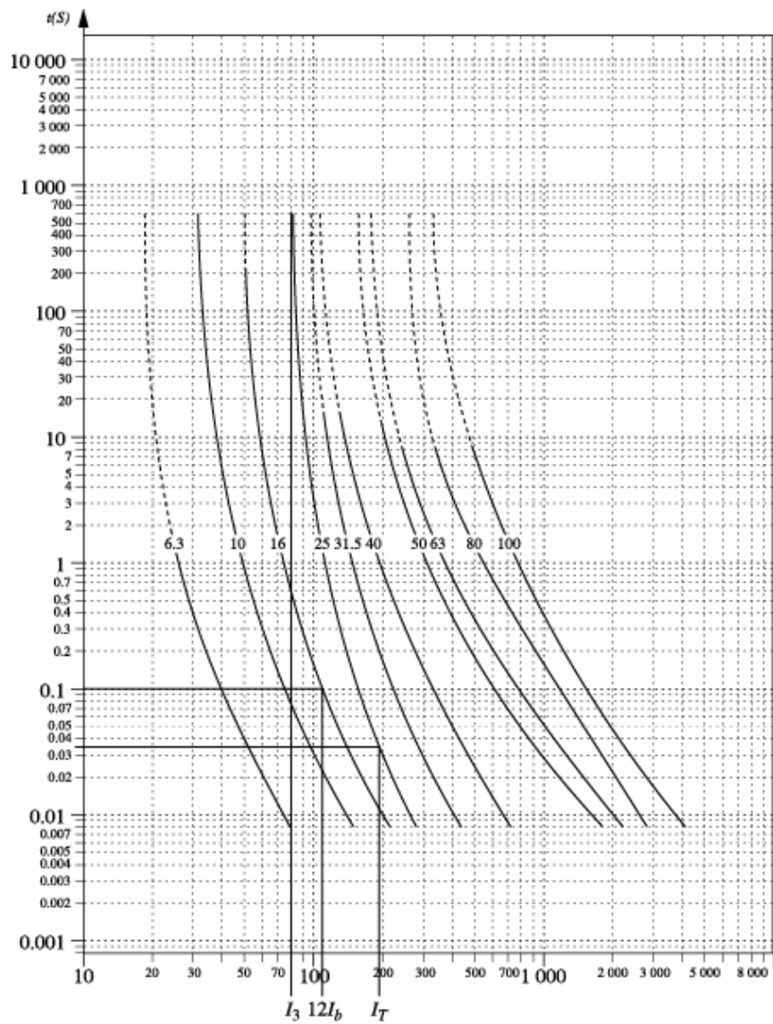
Figure 10-27c: fusing curve – 24 kV internal Fusarc fuse
