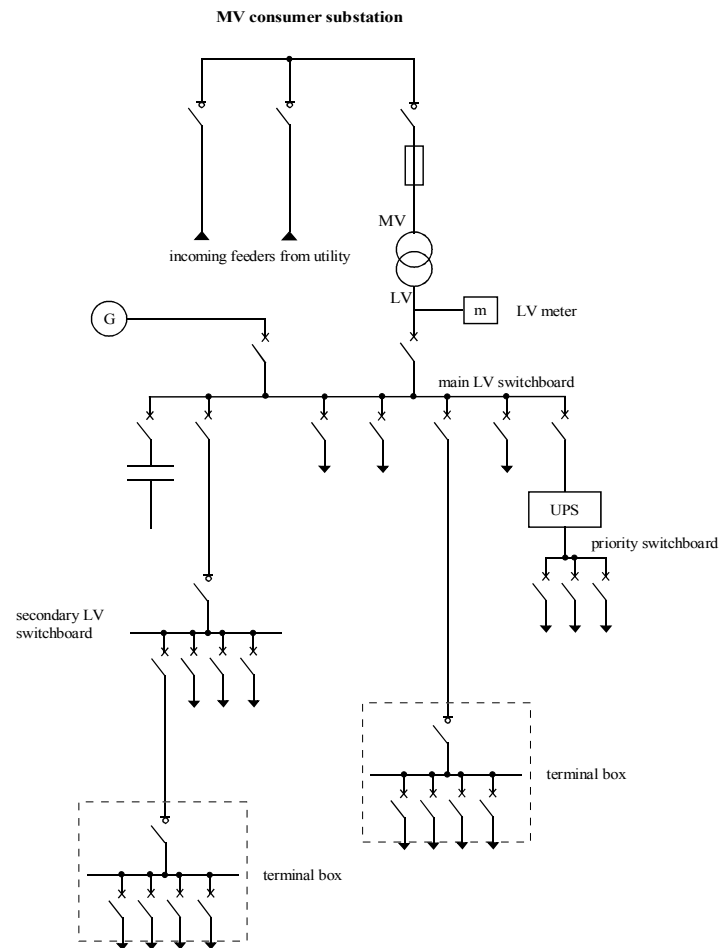
Figure 1-35: example 1
