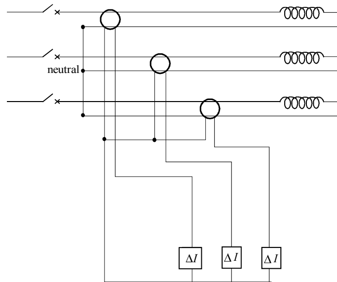
Figure 7-37: motor differential protection with toroids surrounding the upstream and downstream links of each winding
