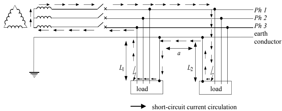
Figure 4-21: fault loop for a double fault on phases 1 and 3 in an IT system without a distributed neutral
