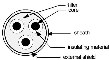
Figure 4-12: collectively shielded cable
