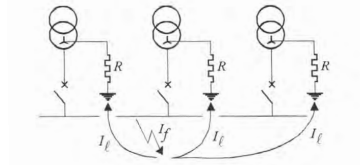
Figure 2-8a: direct earthing of each neutral point
