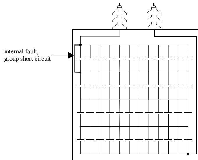
Figure 10-44: capacitor without internal protection fuses
