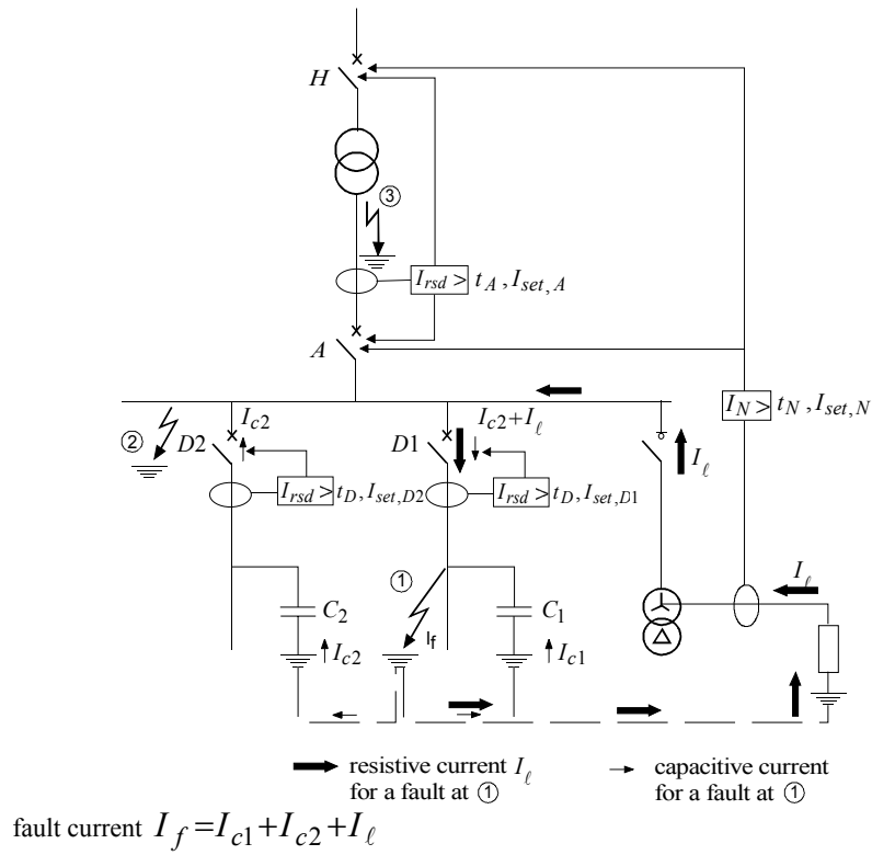
Figure 10-6: neutral earthing via resistor on the busbar
