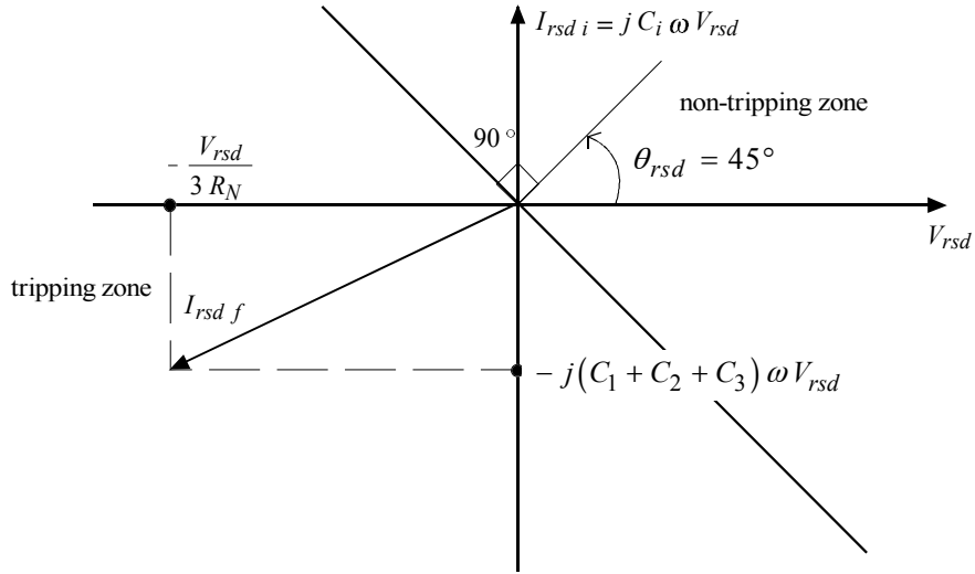
Figure 7-21: phase displacements between residual current and residual voltage detected by the faulty feeder protection and the healthy feeder protection devices
