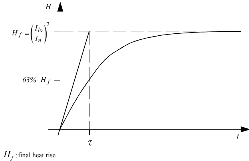
Figure 7-52: loading a machine from a cold state
