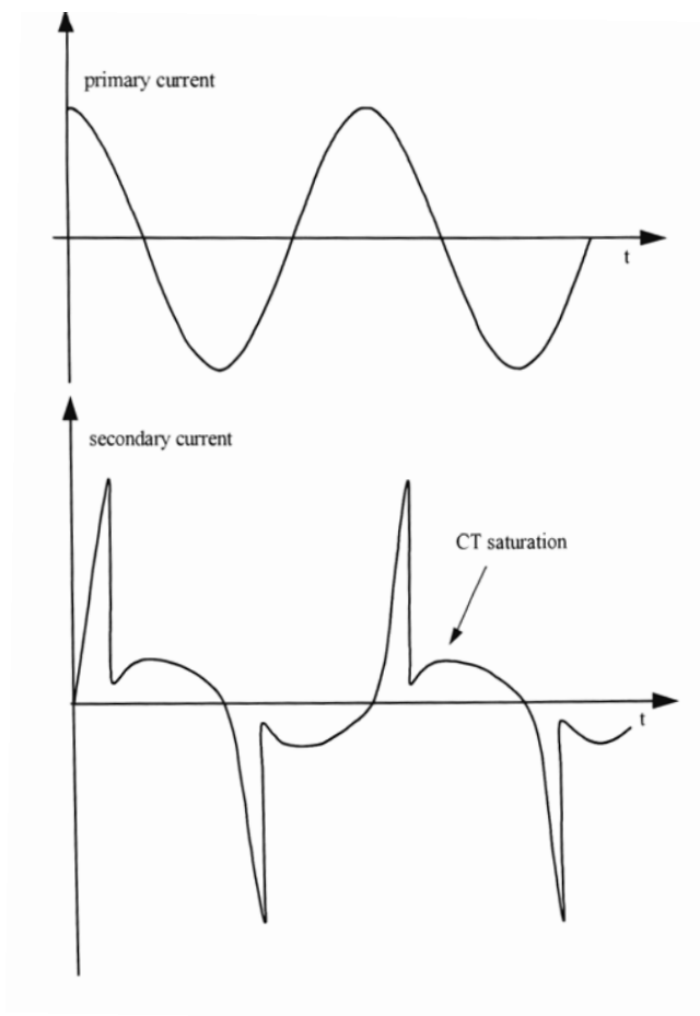
Figure 6-5: secondary current of a current transformer operating under saturated conditions
