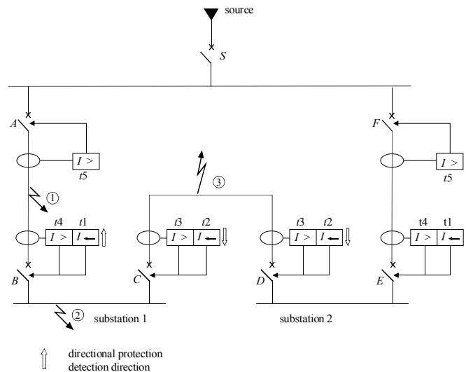
Figure 10-17: solution using overcurrent and directional overcurrent protection devices
