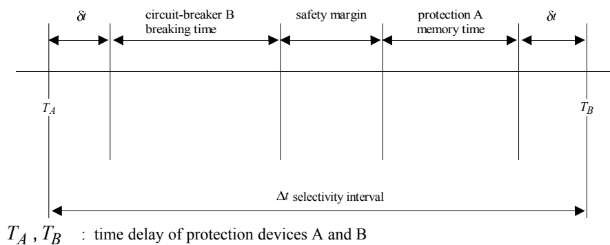
Figure 9-3b: selectivity interval
