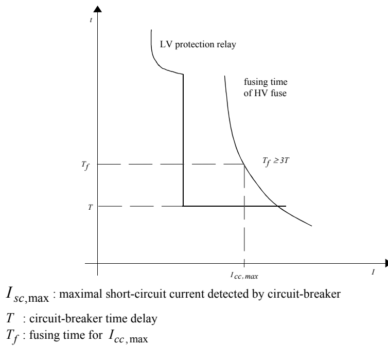
Figure 9-12: Selectivity between MV fuse upstream of a circuit-breaker
