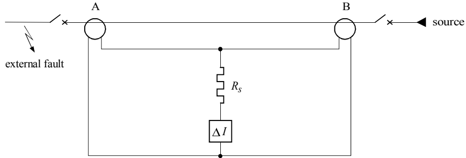
Figure 7-32a: incorporation of a stabilizing resistor in the differential branch
