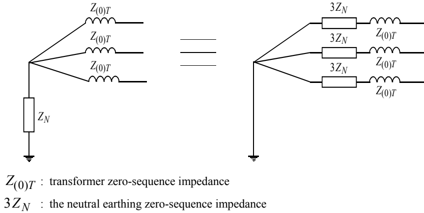
Figure 4-11: neutral earthing zero-sequence impedance
