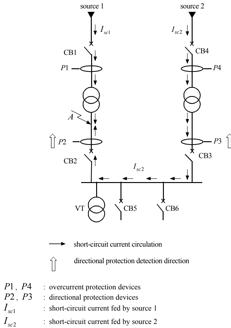
Figure 7-9: dual fed busbar
