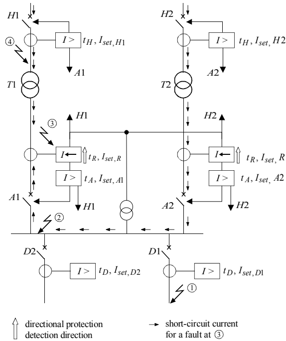
Figure 10-8: protection against phase-to-phase faults
