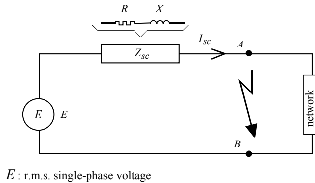
Figure 4-1: equivalent diagram of the network upstream of the short-circuit
