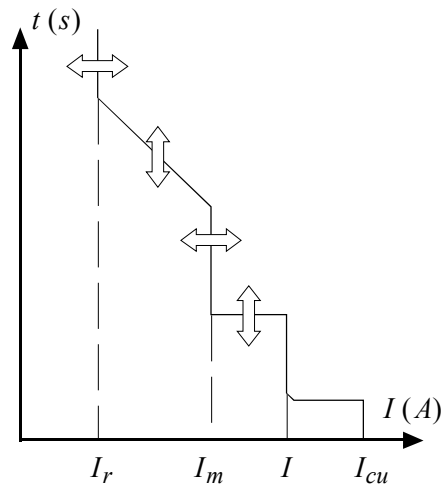
Figure 8-3: standard operating curve for an electronic circuit-breaker
