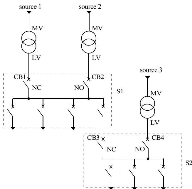
Figure 1-23: dual fed LV switchboards with no coupler
