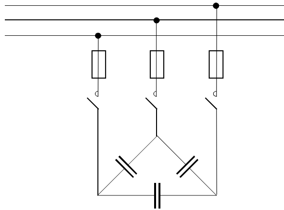
Figure 10-46: delta-connected bank
